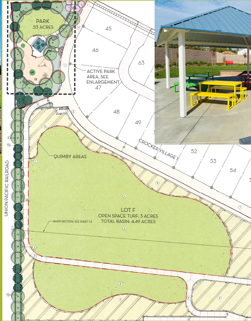
Large Open Turf Area Detention Basin
