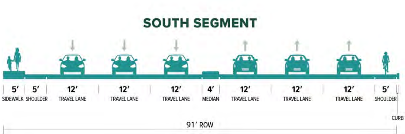
Figure 14. South Segment: Howe Avenue - La Riviera Access Road to Power Inn Station
