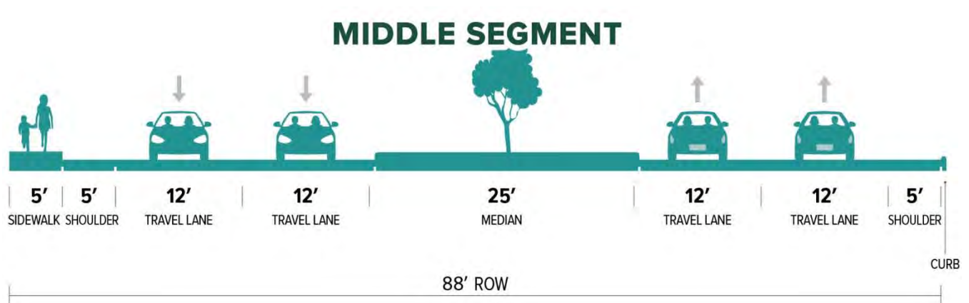
Figure 11. Middle Segment: Howe Avenue (Swarthmore Drive to La Riviera Access Road)
