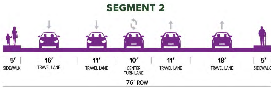
Figure 3. Segment 2: Norwood Avenue (Bell Avenue to I-80)
