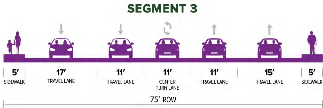
Figure 4. Segment 3: Norwood Avenue (I-80 to Carroll Avenue)
