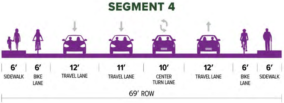
Figure 5. Segment 4: Norwood Avenue (Carroll Avenue to Arcade Creek)
