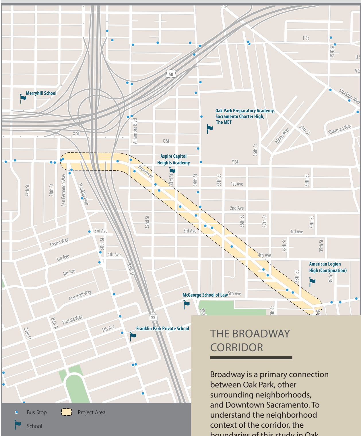
FIGURE 2: STUDY AREA
