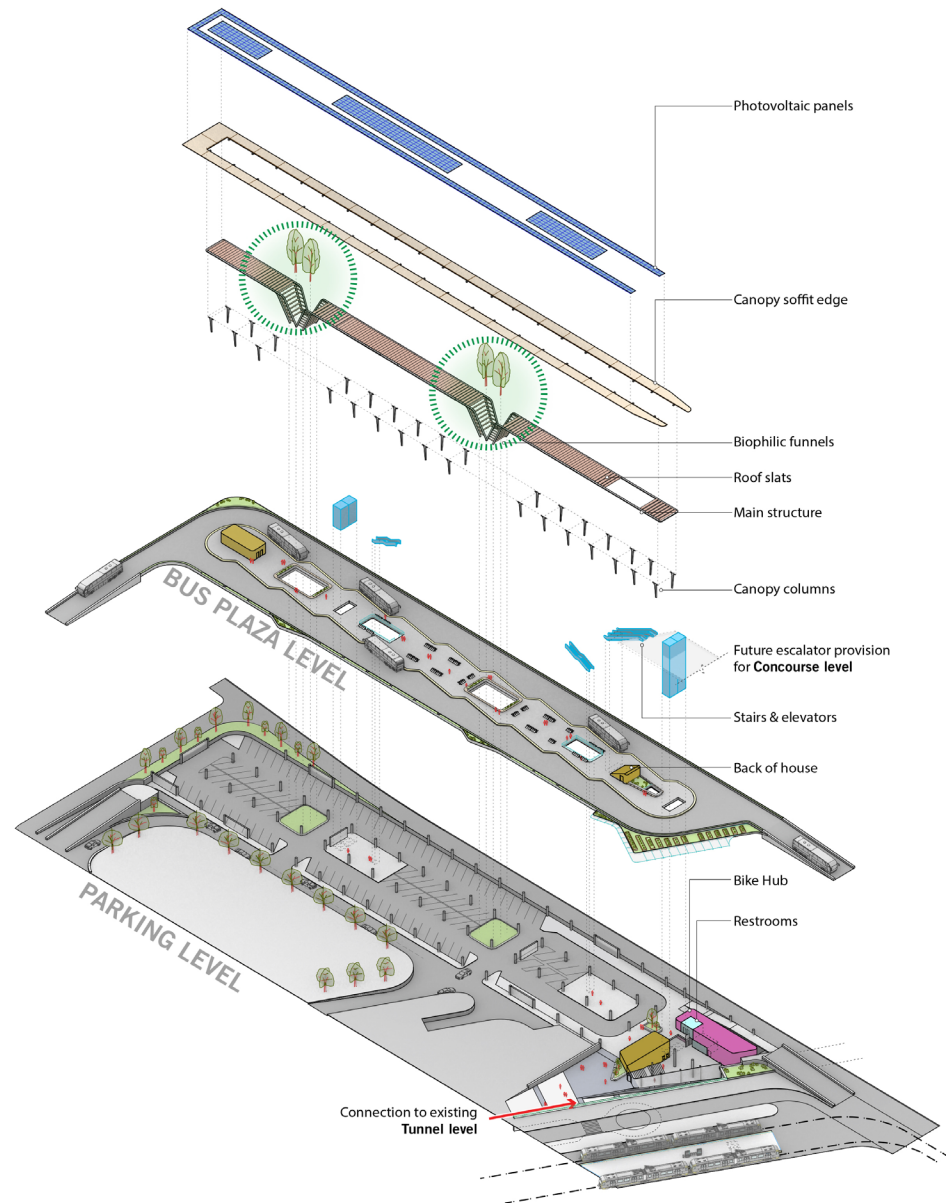
Figure 6.12 Bus Mobility Center Overview
