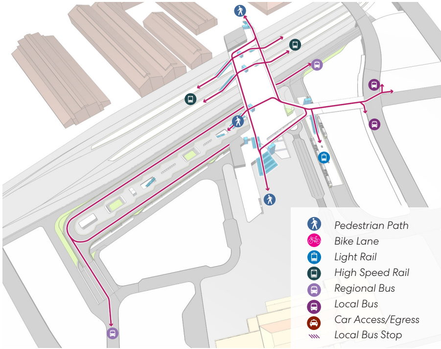
Figure 6.21 Station Access - Concourse Level
