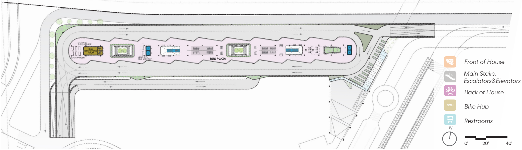
Figure 6.13 Bus Mobility Center Floor Plan - Bus Plaza Level
