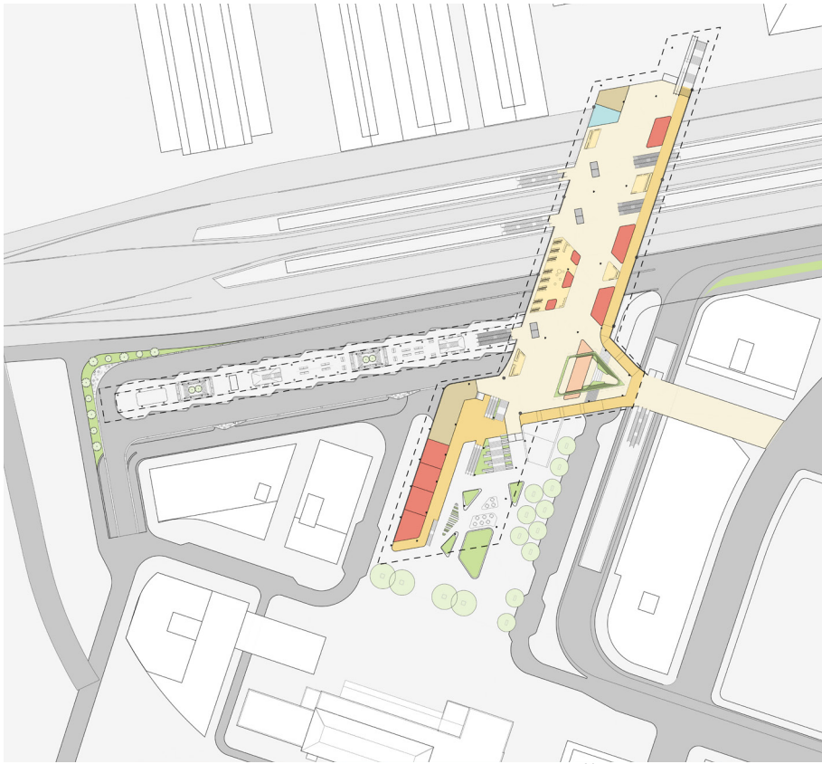
Figure 6.18 Station Plan - Concourse Level
