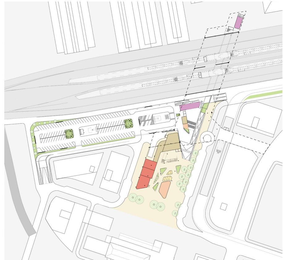
Figure 6.17 Station Plan - Ground Floor
