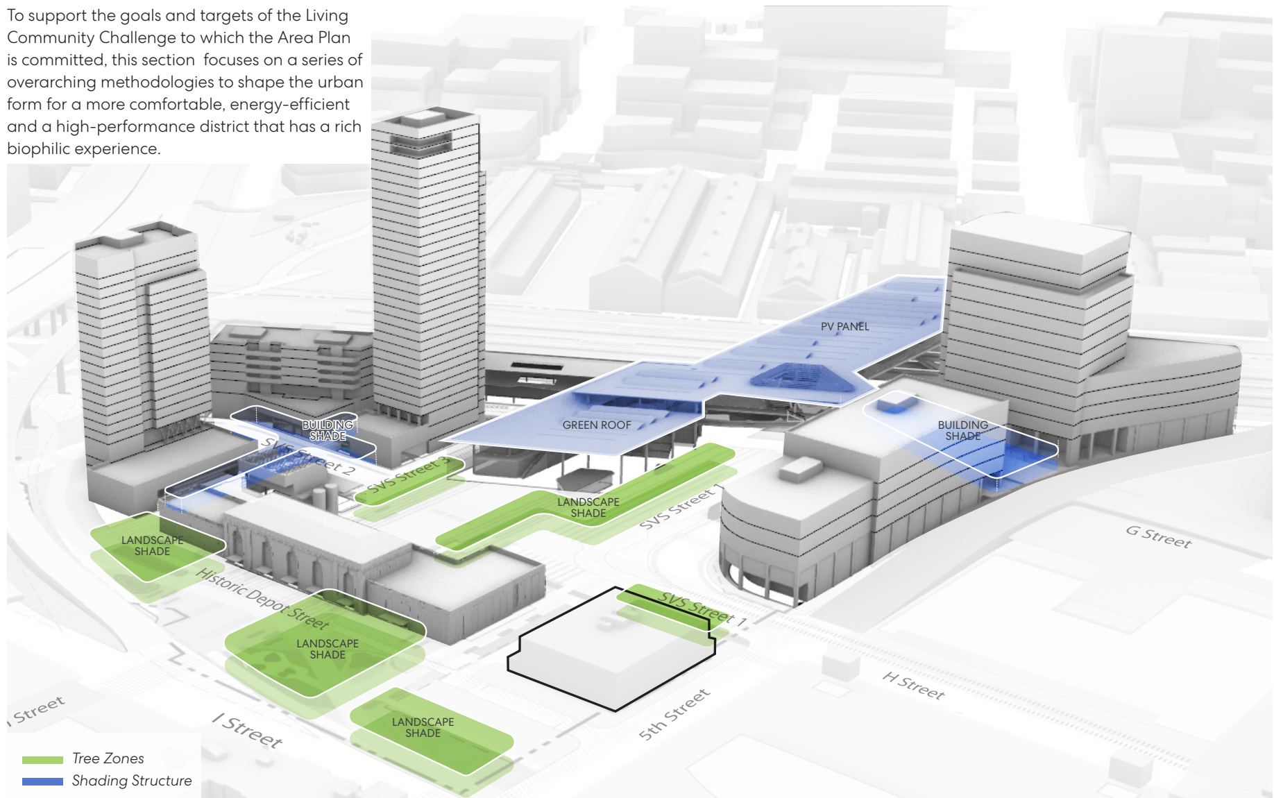
Figure 6.3 Shading Strategy - Cooling the Building Cluster
