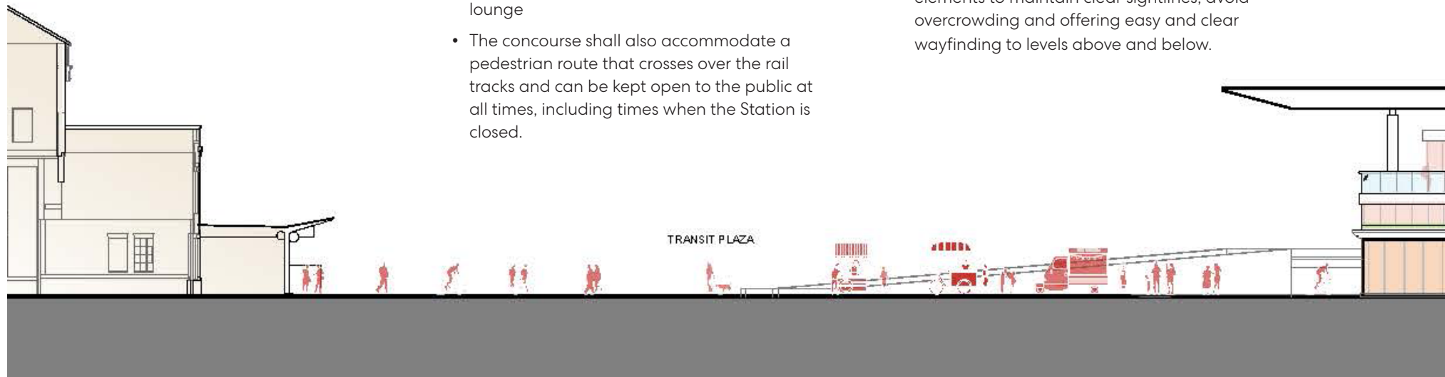
Figure 6.22 Section - A1
