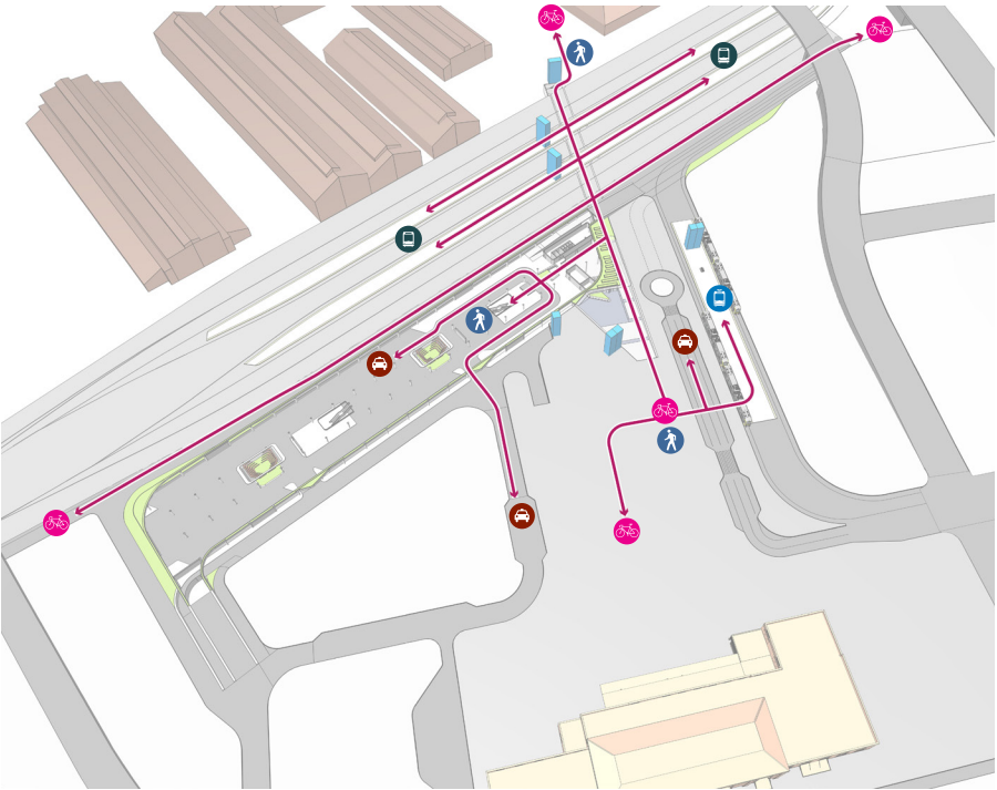
Figure 6.20 Station Access - Ground Level
