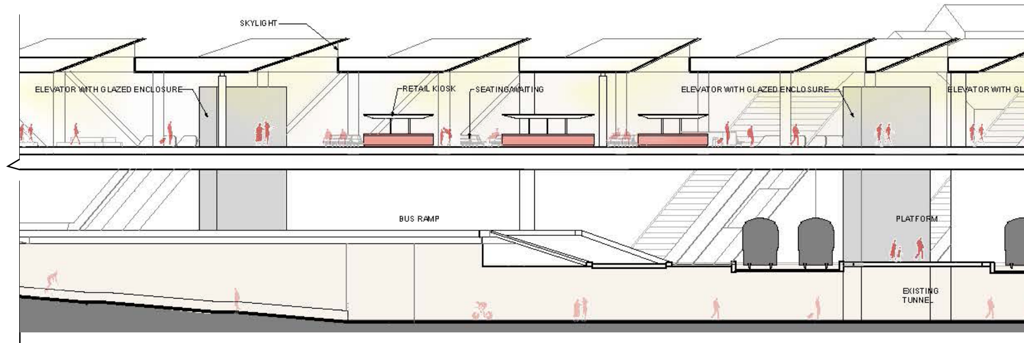
Figure 6.23 Section - A2
