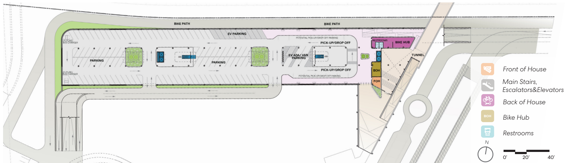
Figure 6.14 Bus Mobility Center - Plan - Parking Level
