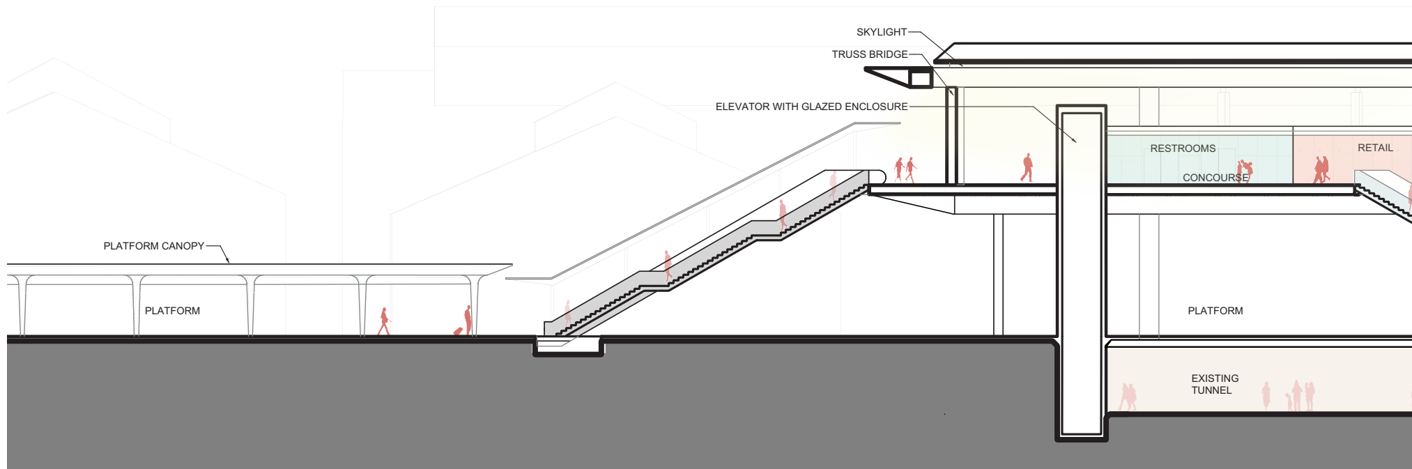
Figure 6.24 Section - B
