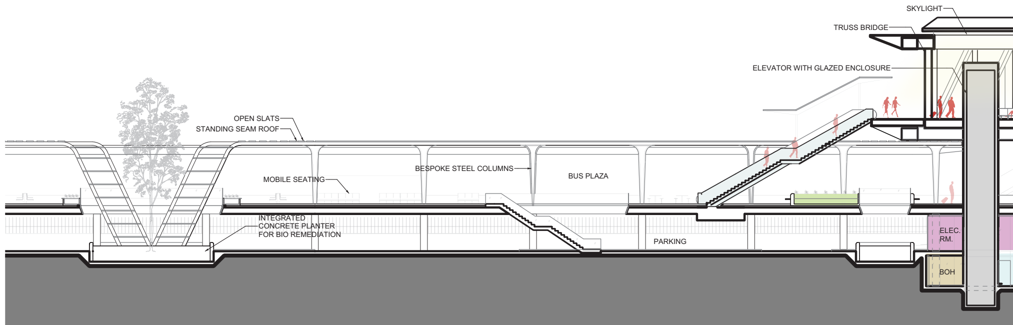
Figure 6.25 Section - C
