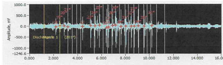
Sensor 23 (456m)
