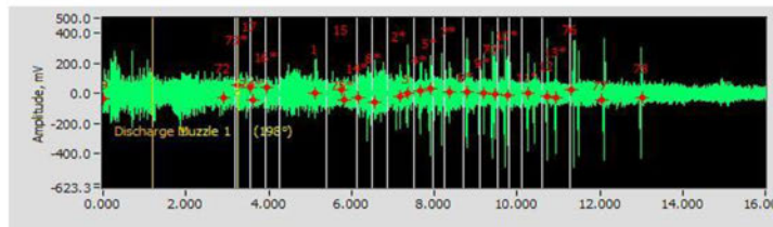
Sensor 22 (706m)
