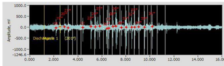
Sensor 23 (456m)
