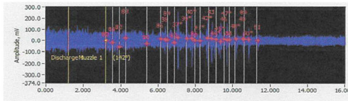
Sensor 25 (668m)
