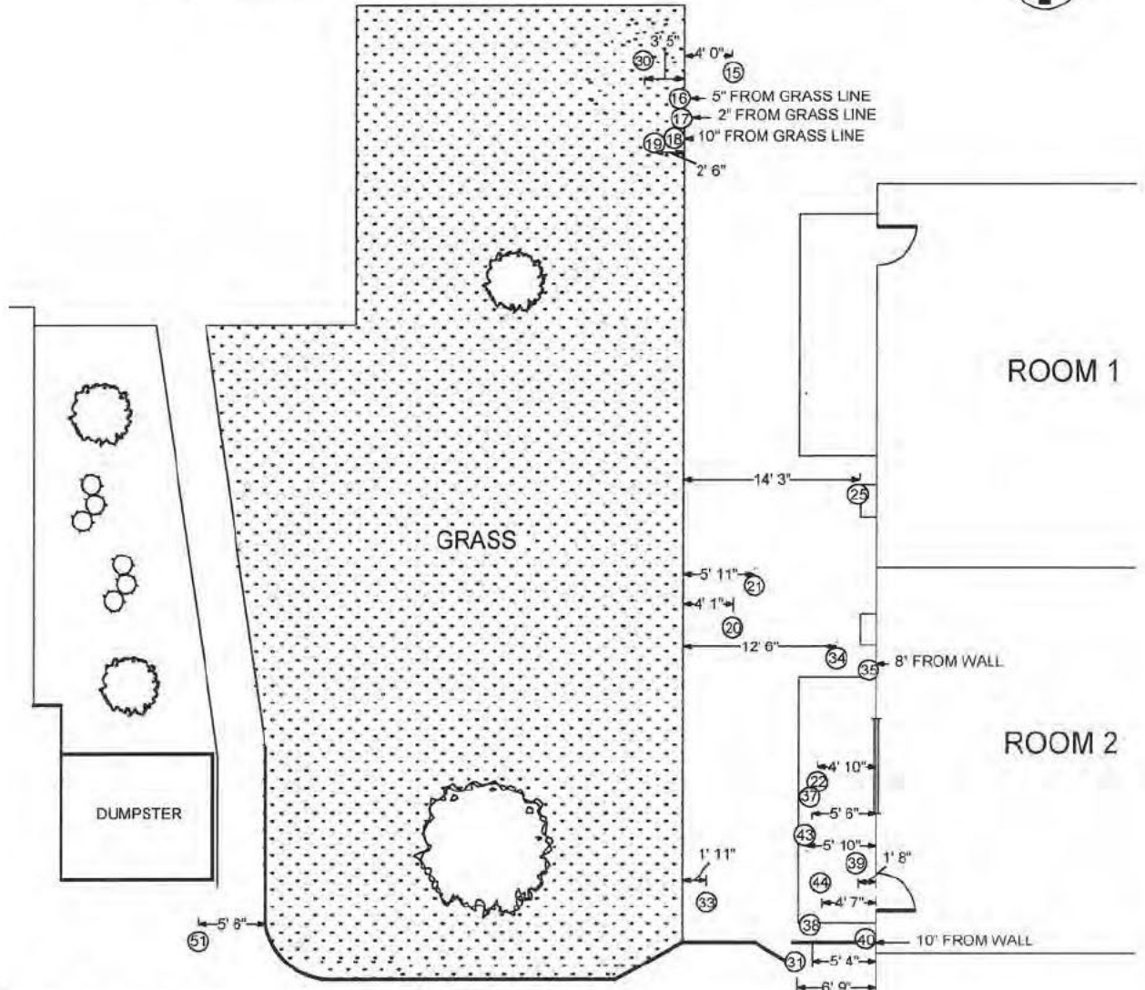
DIAGRAM #7 B EAST/WEST MEASUREMENTS OF ITEMS #15 THRU 22, 25, 30 THRU 35, 37 THRU 40, 43, 44, AND 51
