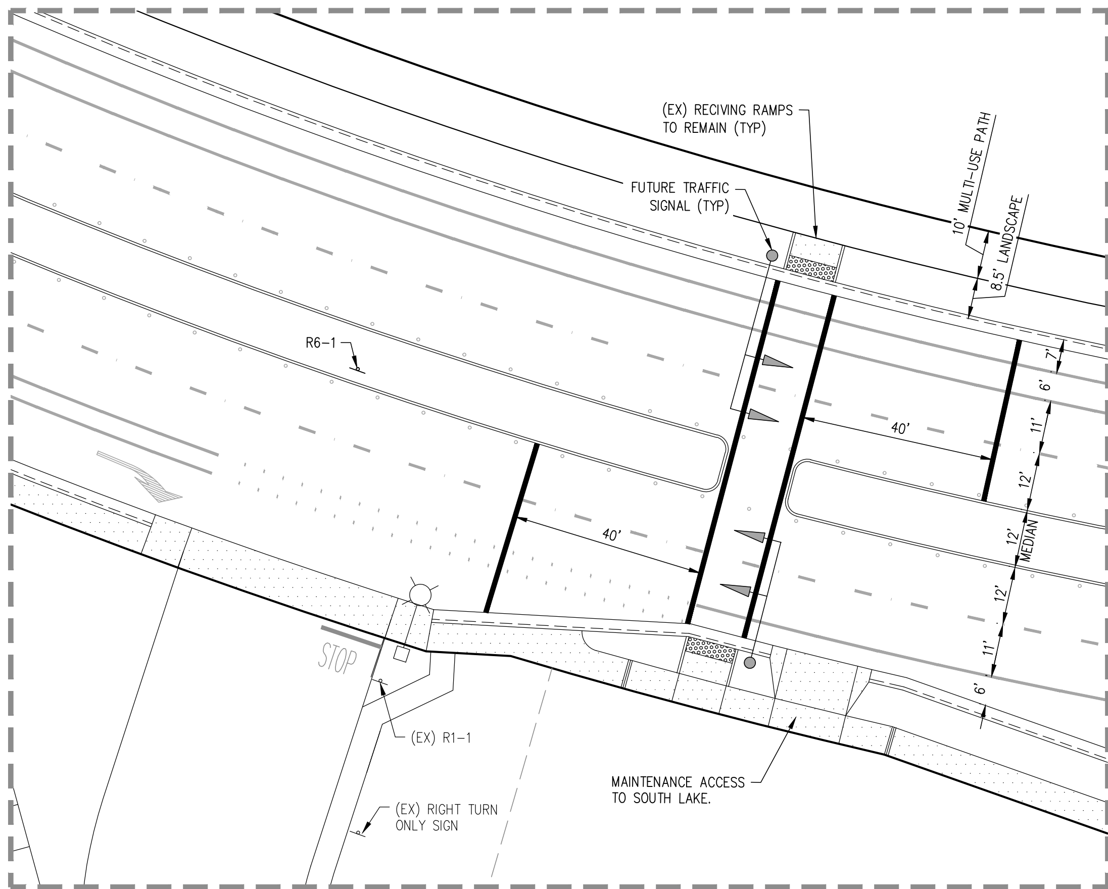
DETAIL B SCALE: 1"=20'
