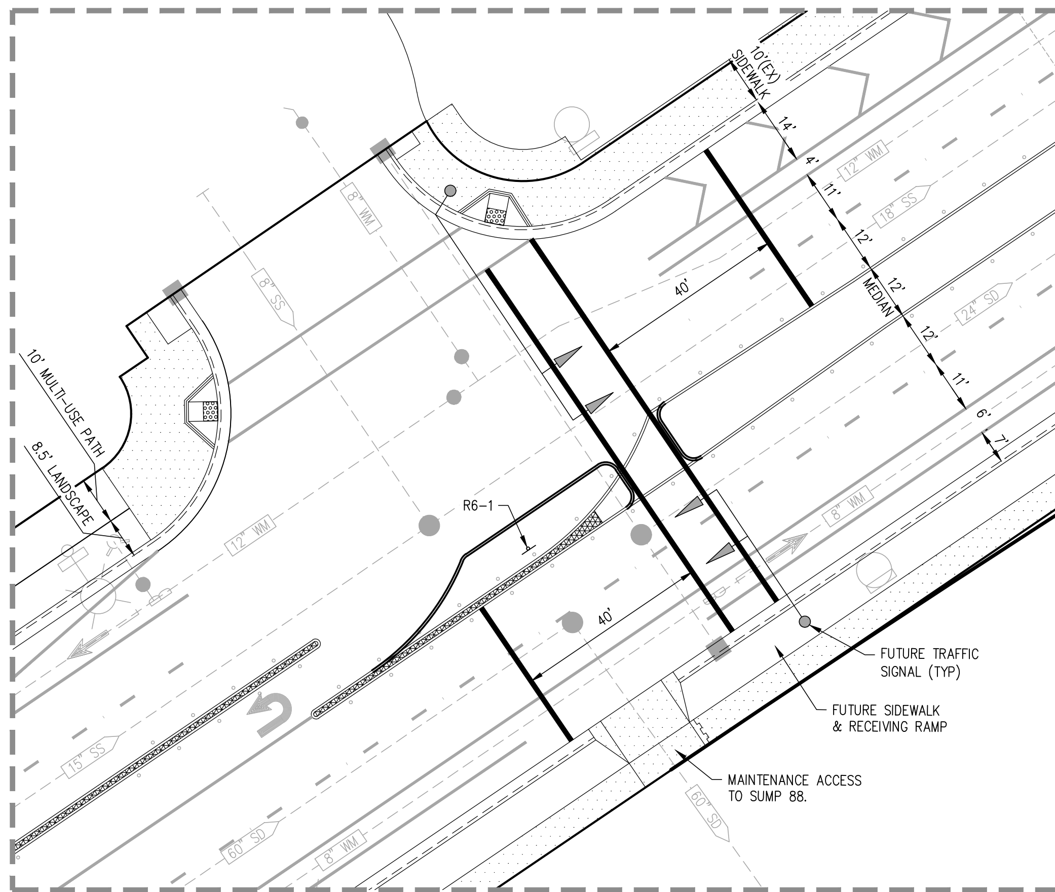
DETAIL C SCALE: 1"=20'
