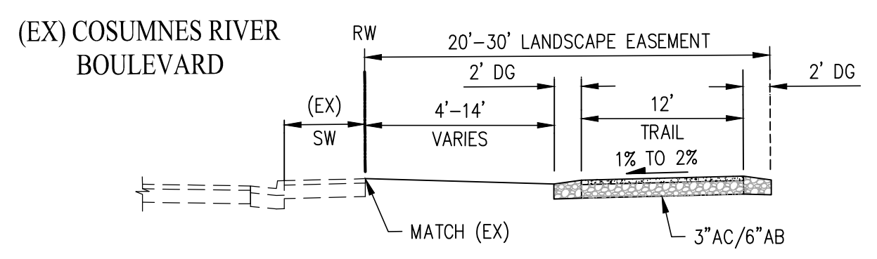
TYPICAL TRAIL SECTION NOT TO SCALE
