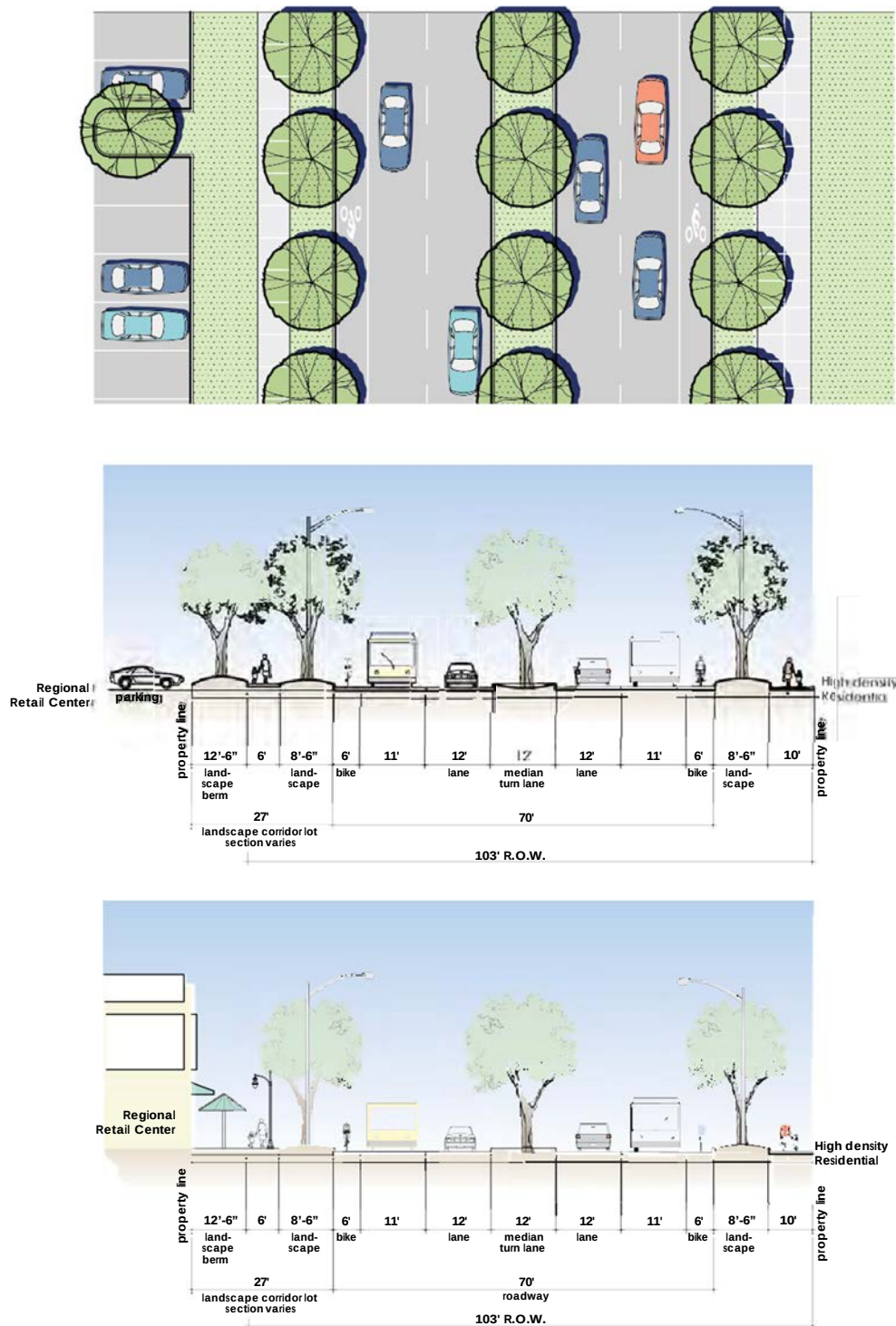
Figure 6.3: Delta Shores Circle North and South (Along Regional Retail Center and Village Center)
