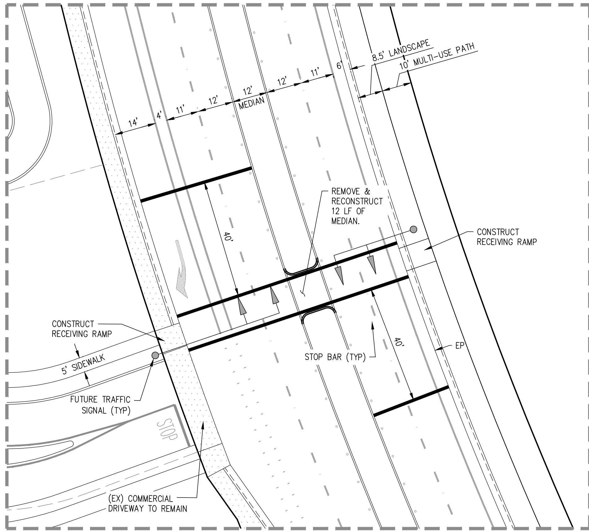
DETAIL A SCALE: 1"=20'
