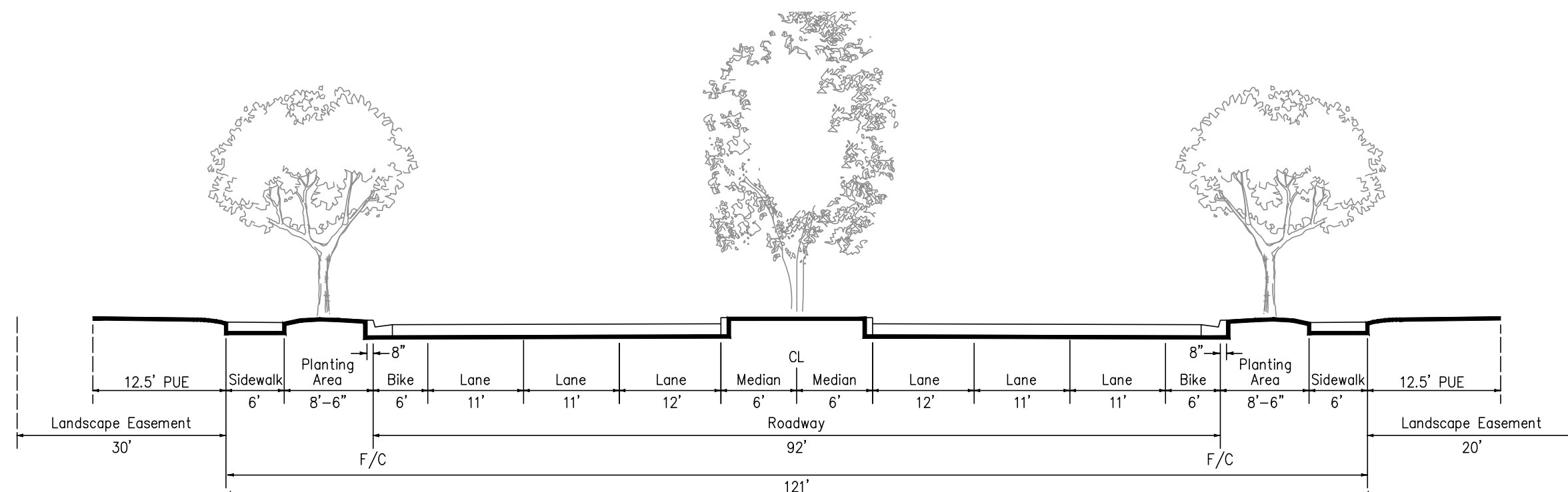
COSUMNES RIVER BOULEVARD (6-LANE)
