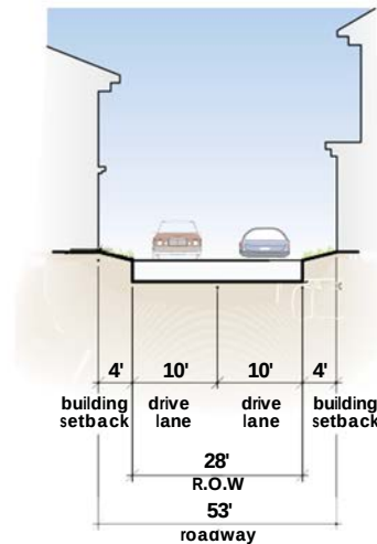
Figure 6.10: Typical Alley
