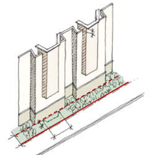
Figure 3. Bay Windows projecting over the setback line. They should be at least 6' apart.
