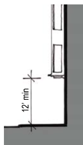
Figure 2. Bay Window - minimum clear height above finished sidewalk
