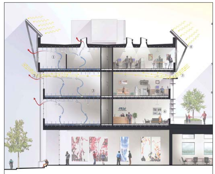
Figure 5. Cross section of an office building showing integrated ventilation and daylighting strategies.
