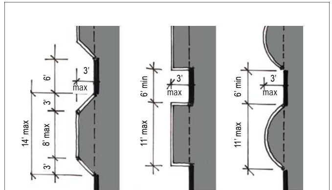
Figure 1. Bay Windows (plan views), left to right: segmented, square, and curved
