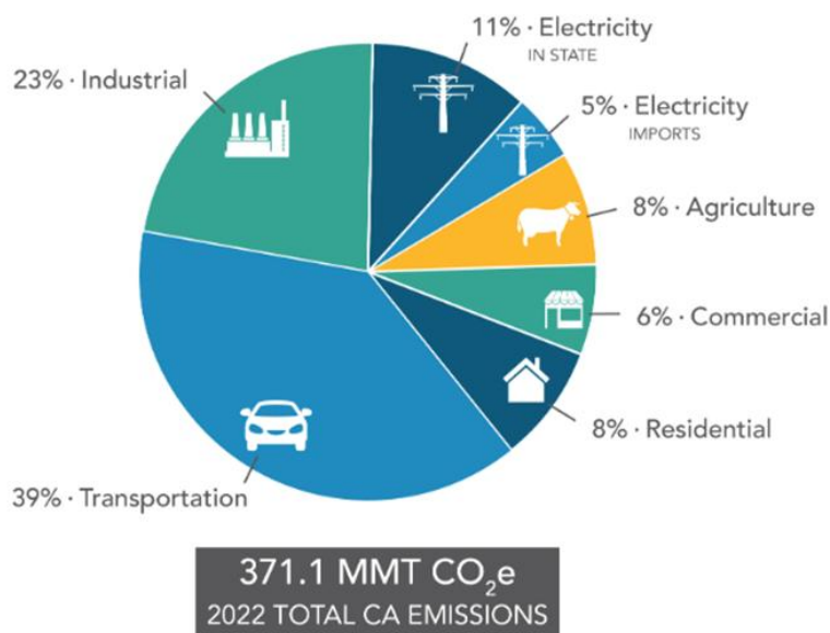
Figure 10. California Greenhouse Gas Inventory
