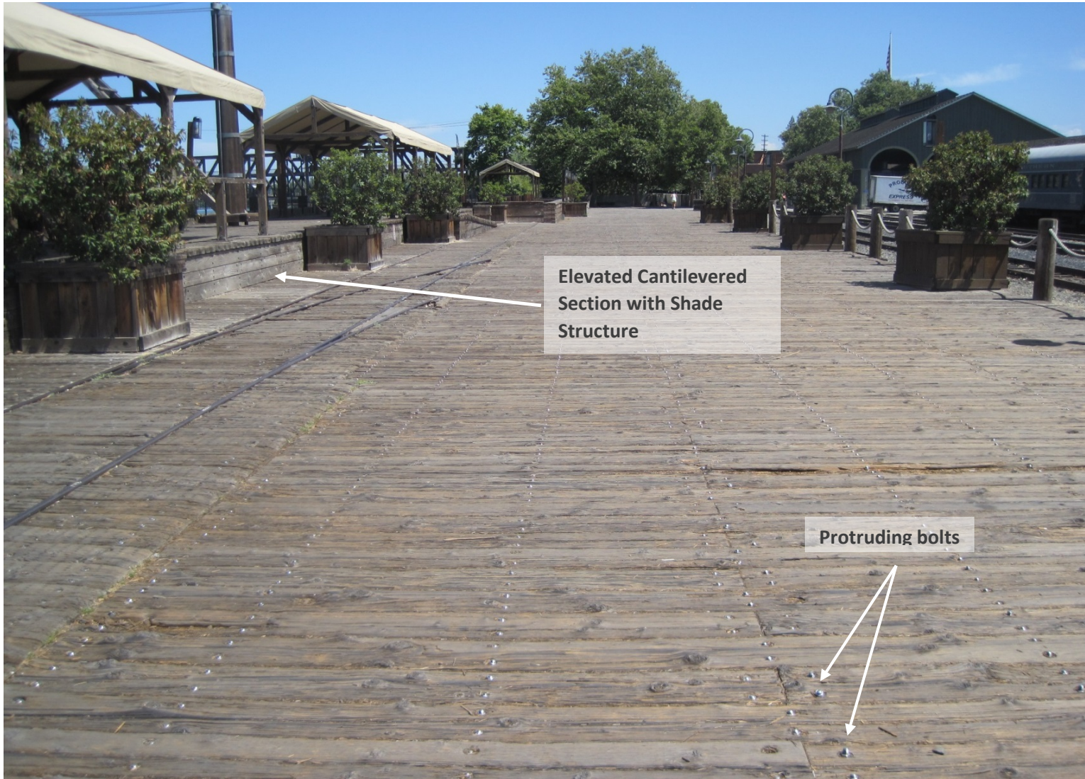
Existing Wood Deck on the Embarcadero with Protruding Bolts.
