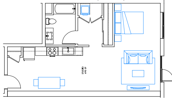
STUDIO 490 SF 1/4" = 1'-0"
