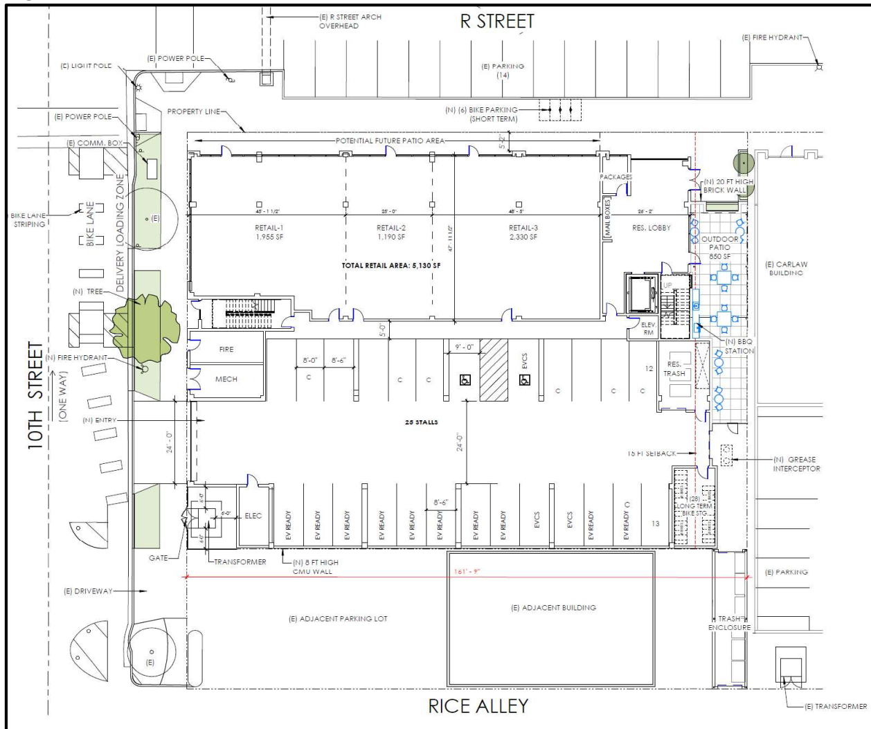
Figure 2: Site Plan
